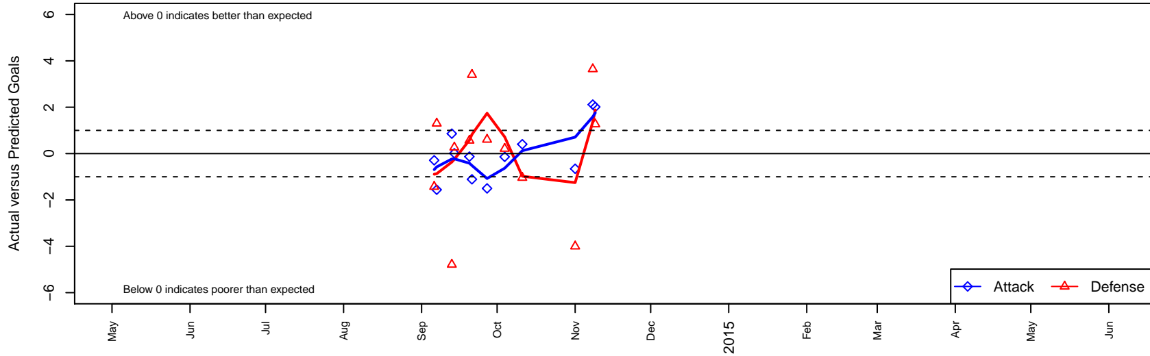
BSC Hood River Vapor G02 Dots are actual minus expected GF (blue circles) and GA (red triangles). Blue line is smoothed change in attack strength. Red is smoothed change in defense strength.
